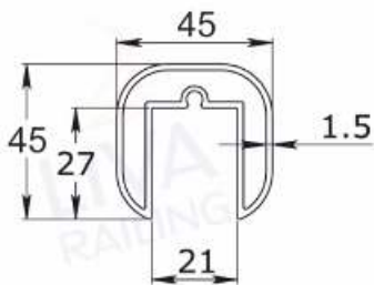
Wall Conceal
