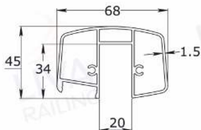
Wall Conceal
